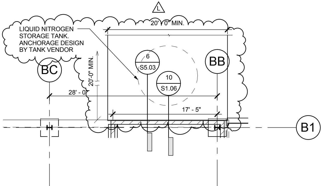
1 LN TANK FOUNDATION - PLAN 1/8" = 1'-0"
