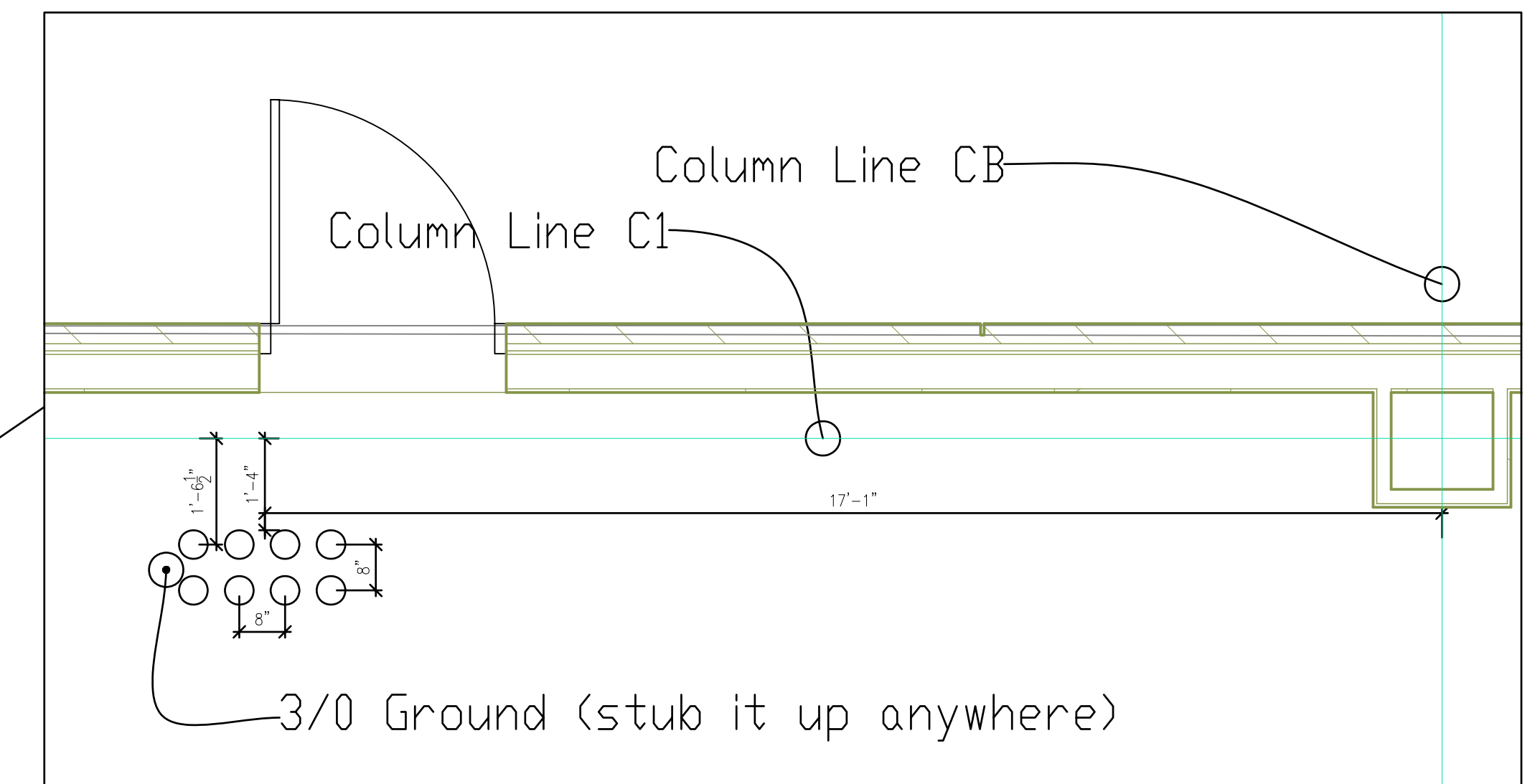
CSF Room 1811 Scale: 1"=4'
