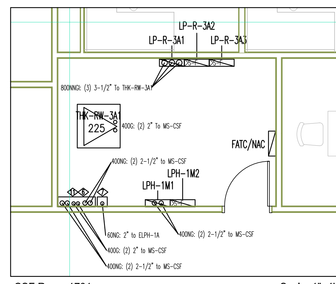
CSF Room 1731 Scale: 1"=4'
