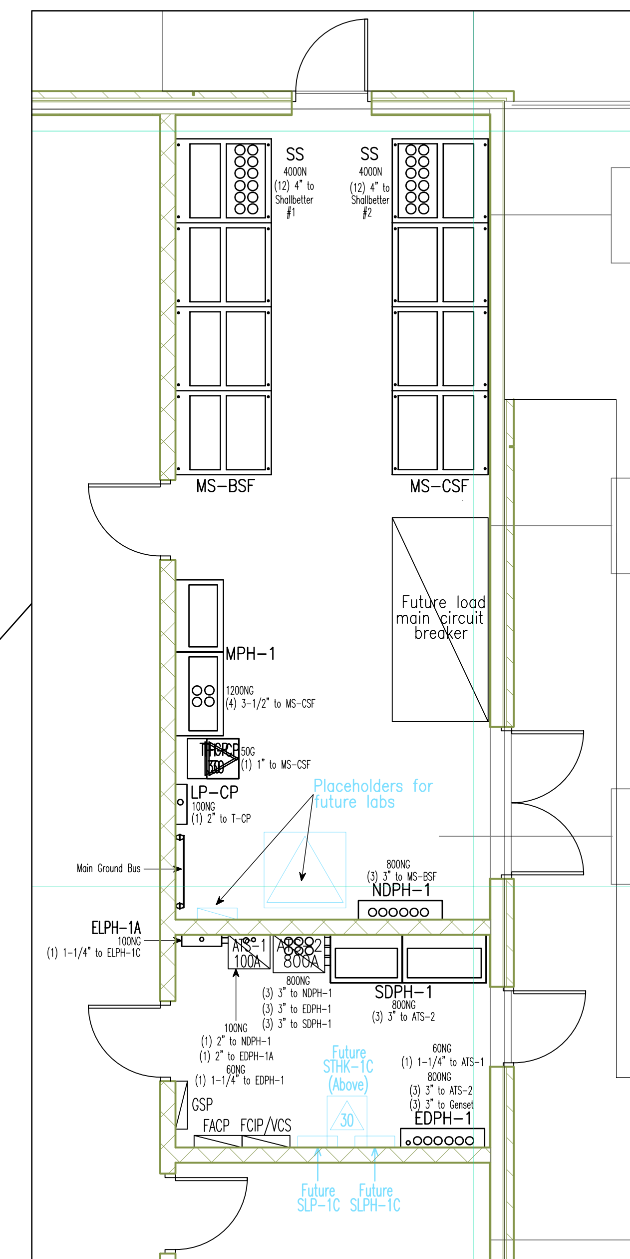
BSF Rooms 1220 & 1222 Scale: 1"=4'
