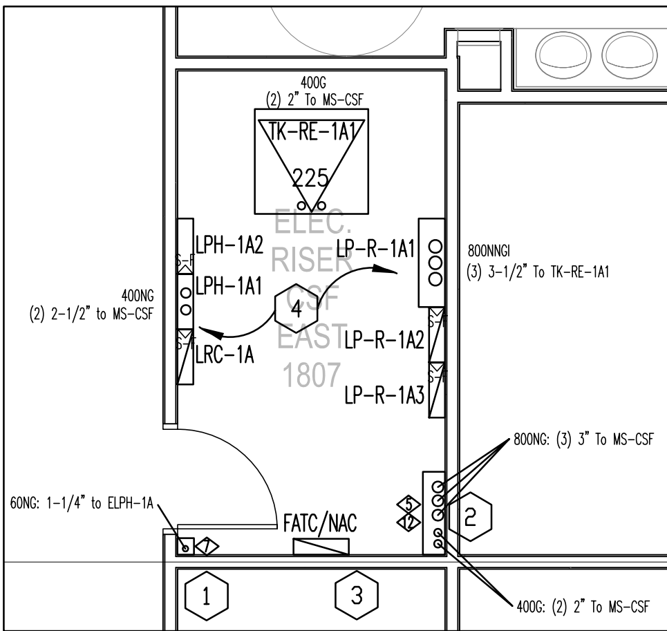
Electrical Room 1807
