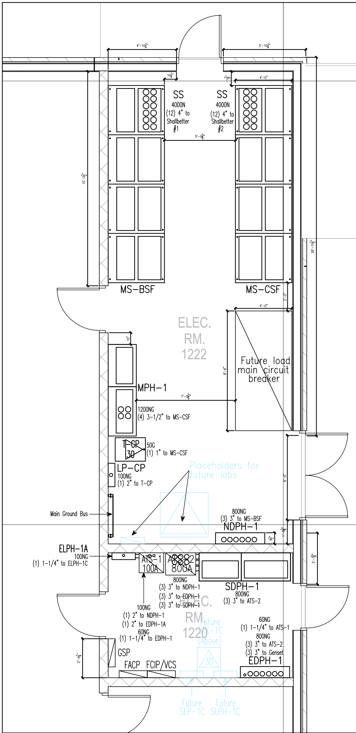
Electrical Rooms 1220 & 1222
